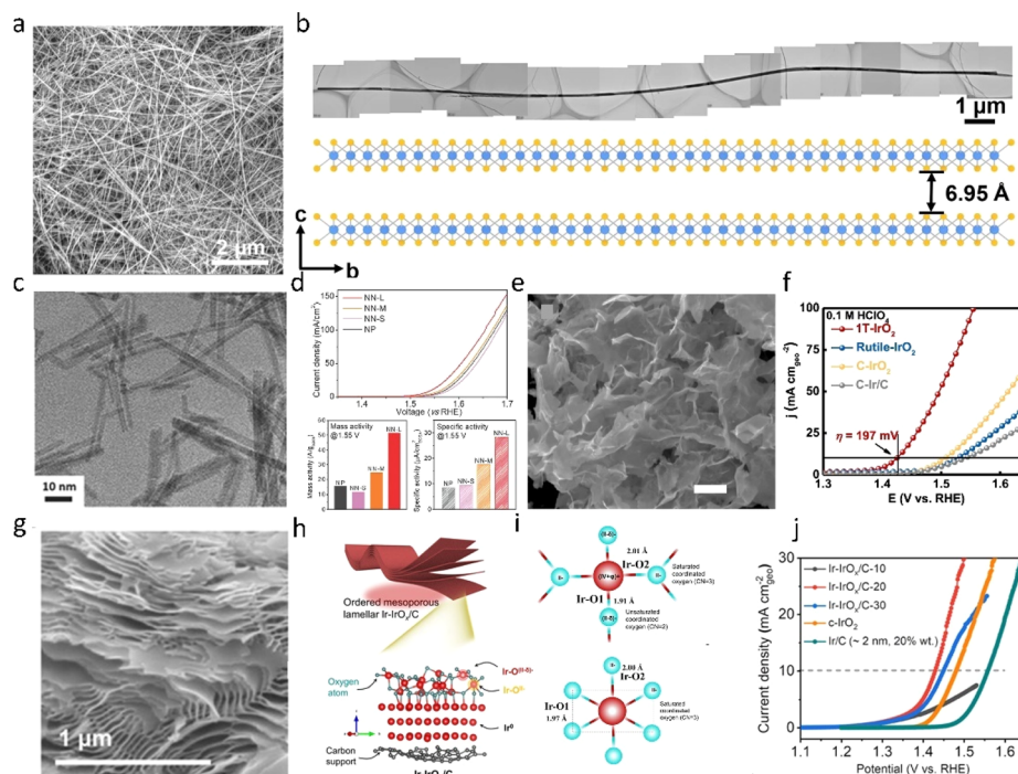
Fig. 5 (a) SEM image showing the uniform distribution of the \text{IrO}_2\text{NR} . (b) A typical long \text{IrO}_2\text{NR} with a length of 22.53 \mu\text{m} . 51 Copyright 2023, Springer Nature. (c) TEM image of \text{IrO}_2 nanoneedles. (d) Initial OER performance of \text{IrO}_2 . 57 Copyright 2017, Wiley-VCH. (e) The SEM image of 1T- \text{IrO}_2 , showing its ultrathin morphology. (f) Polarization curves of 1T- \text{IrO}_2 , rutile- \text{IrO}_2 , and commercial catalysts (C- \text{IrO}_2 and C-Ir/C) in \text{O}_2 -saturated 0.1 \text{ M HClO}_4 electrolyte with iR -correction. 58 Copyright 2021, Springer Nature. (g–i) The nanosheet structure of 2D \text{IrIrO}_x/\text{C}-20 . (j) Water oxidation polarization curves recorded with a linear scan of potential at 2 \text{ mV s}^{-1} for Ir- \text{IrO}_x/\text{C} , commercial crystalline c- \text{IrO}_2 , Ir/C, and carbon black. 59 Copyright 2022, American Chemical Society.
