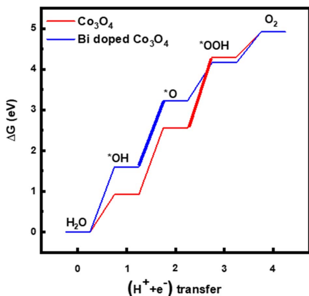
Fig. 7 Diagrams showing calculated free energy changes of OER on the surface of Co 3 O 4 (100) and Bi-doped Co 3 O 4 .
