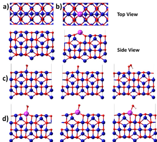
Fig. 6 Top view and side view images of (a) Co 3 O 4 (100) surface and (b) Bi-doped Co 3 O 4 (100) surface. Red: oxygen, blue: cobalt, and purple: bismuth. Optimized structures of (c) Co 3 O 4 (100) surface and (d) Bi-doped Co 3 O 4 (100) surface, with both showing surface-adsorbed *OH, *O, and *OOH intermediates.
