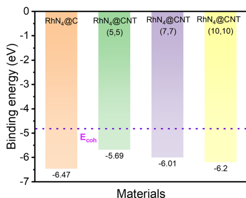
Fig. 2 The calculated cohesive energy of Rh and the binding energy ( E_b ) of \text{RhN}_4\text{@C} and \text{RhN}_4\text{@CNT}(n, n) ( n = 5, 7, 10 ).
