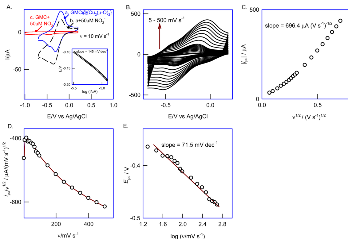
Fig. 7 (A) Comparative CV responses of GCE/GMC@{Cu 2 (μ-O) 2 } without (curve a) and with 50 μM NO 2 - (curve b), GCE/GMC (curve c), at scan rate ( ν ) = 10 mV s -1 ; and inset is a Tafel plot. (B) Effect of scan rate ( ν ) on the GCE/GMC@{Cu 2 (μ-O) 2 } from 5 to 500 mV s -1 , in the presence of 50 μM NO 2 - ; plots of (C) i pc vs. ν 1/2 , (D) i pc ν 1/2 vs. ν and (E) E pc vs. log( ν ). Electrolyte: nitrogen purged 0.1 M PBS, pH 7.
