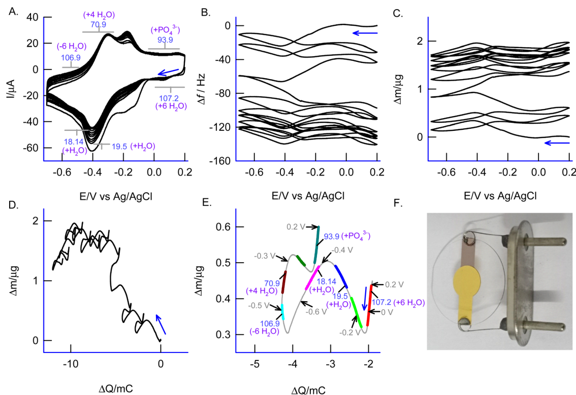
Fig. 5 (A and B) In situ CV-EQCM responses of GCE/GMC@ \{\text{Cu}(\text{BPA})\text{Cl}\}_{\text{ads}} in \text{N}_2 purged 0.1 M PBS, pH 7, at a scan rate of 10\text{ mV s}^{-1} . Inset of (A) shows the molecules involved in the redox reaction. Corresponding derivative plots of (C) \Delta m vs. E and \Delta m vs. \Delta Q plots of (D) 1–10 cycles and (E) second cycle. (F) Picture of an EQCM-Au electrode.
