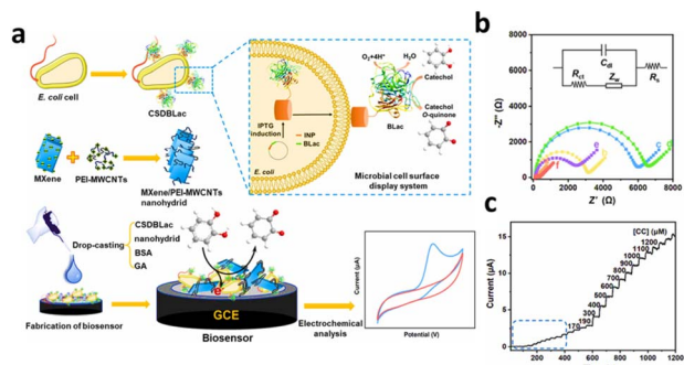
Fig. 9 (a) The CSDBLac and biosensor application and construction schematics. (b) GCE's impedance spectrum (b(a)), CSDBLac/GCE (b(b)), GA-CSDBLac/GCE (b(c)), GA-BSA-CSDBLac/GCE (b(d)), GA-BSA-MXene-CSDBLac/GCE (b(e)) and GA-BSA-MXene-PEI-MWCNTs-CSDBLac/GCE (b(f)). (c) CC's magnification curves. Reprinted from ref. 133, copyright (2023), with permission from Elsevier.
