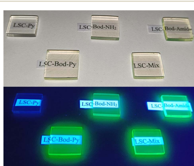
Fig. 3 Photograph of the prepared LSC before and after UV irradiation at 365 nm.
