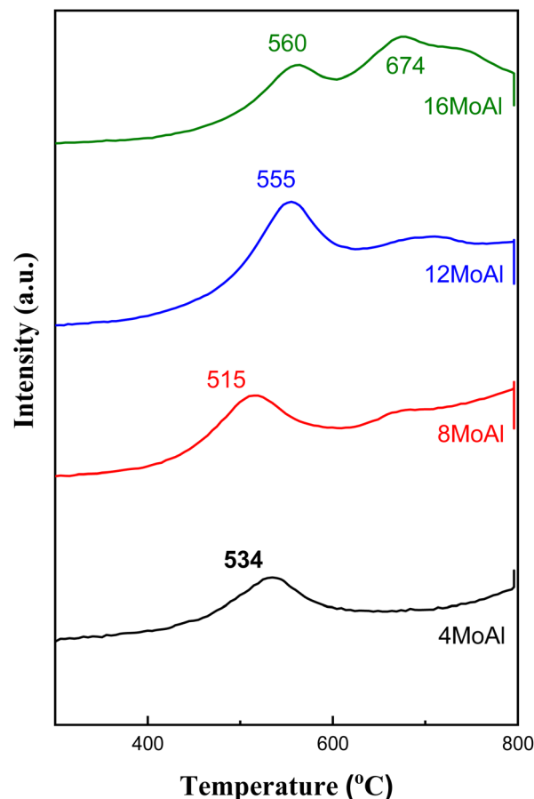
Fig. 5 H 2 TPR profile of the catalysts with varying Mo-loading on \gamma -Al 2 O 3 .
