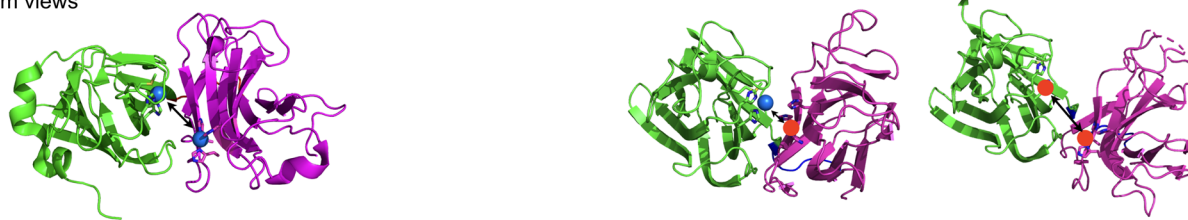
Fig. 2 Uncoupled binuclear copper-containing monooxygenases, PHM and D \beta H. (a) and (b) reactions catalyzed by PHM and D \beta H, respectively; (c) X-ray structure of PHM from Rattus norvegicus showing the two domains (Cu M domain in green and Cu H domain in magenta) connected by a loop (in blue) in which each domain binds a single copper atom spaced from each other by approximately 11 Å and (d) structure of the Cu M -superoxido intermediate in PHM (PDB ID 1opm); (e) and (f) X-ray structure of the human D \beta H (PDB ID 4zel) showing the open (e) and the closed (f) forms. Only the Cu M domain of the closed form contains a copper atom, the other copper ions (red sphere) are manually placed.
