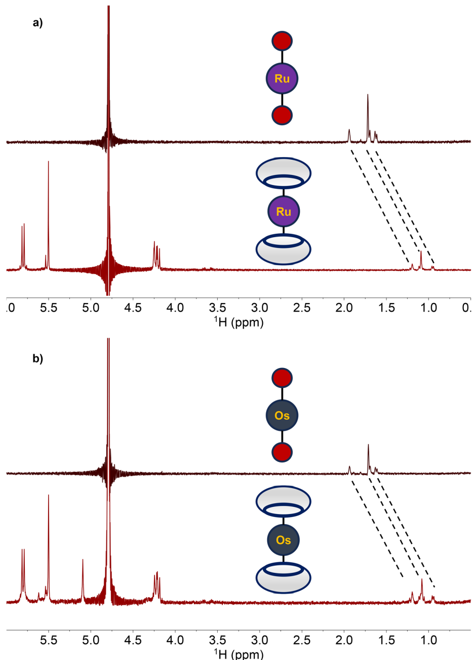
Fig. 2 (a) ^1\text{H} NMR (500 MHz, 25 ^\circ\text{C} ) spectra in \text{D}_2\text{O} of 1 (top) and 1 + two equiv. CB[7] (bottom). (b) ^1\text{H} NMR (500 MHz, 25 ^\circ\text{C} ) spectra in \text{D}_2\text{O} of 2 (top) and 2 + two equiv. CB[7] (bottom). The shift of the adamantane ^1\text{H} resonances are indicated with the dotted lines.
