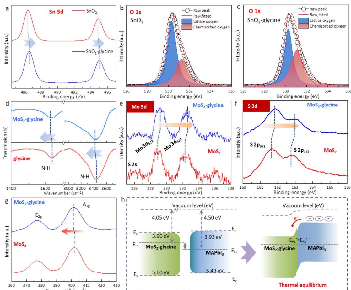
Fig. 6 Interactions between glycine, SnO 2 , and MoS 2 . (a) XPS spectra of the Sn 3d signals of SnO 2 and SnO 2 -glycine. (b and c) XPS spectra of the O 1s of SnO 2 and SnO 2 -glycine. (d) FTIR spectra of glycine and MoS 2 -glycine. (e and f) XPS spectra of the Mo 3d and S 3d signals for MoS 2 and MoS 2 -glycine, respectively. (g) Raman shifts of MoS 2 and MoS 2 -glycine. (h) Schematic diagram of the bandgap alignment at the MoS 2 -glycine/MAPbI 3 interface.
