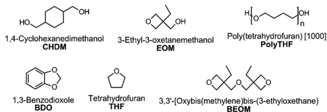
Fig. 7 Carbon-based coiniciators which are suitable to achieve stable frontal polymerization.
