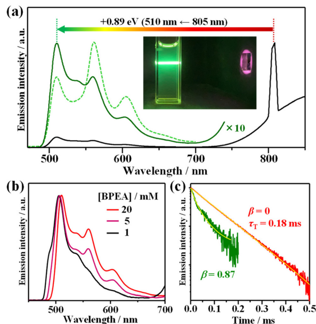
Fig. 4 (a) Upconversion (UC) emission spectra of a mixture containing AuCu-rod (50 \mu\text{M} ) and BPEA (20 mM) in deaerated THF, observed under continuous wave 805 nm laser excitation ( 5.1 \text{ W cm}^{-2} ), and a photographic image of the UC emission captured without any filters. The dashed line represents the UC spectrum of the mixture measured before BPEA reached dissolution equilibrium. (b) UC spectra of mixtures containing AuCu-rod (50 \mu\text{M} ) and BPEA at concentrations of 1, 5, and 20 mM. (c) UC emission decay curves obtained using appropriate filters for either monomer UC emission ( \lambda \leq 525 \text{ nm} , solid green line) or aggregate UC emission ( \lambda \geq 625 \text{ nm} , solid red line). The yellow solid lines represent least-square fitting curves obtained using eqn (3).
