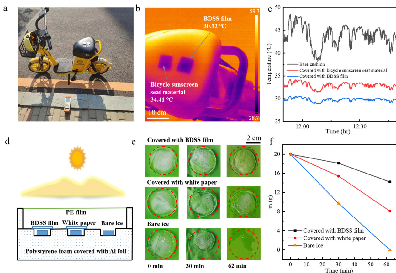
Fig. 4 BDSS film cooling test of actual objects. (a) Device for the cooling test of the shared electric bicycle cushion. (b) The infrared image presenting the cushion from left to right: the cushion covered with bicycle sunscreen seat material, the exposed cushion, and the cushion covered with the BDSS film. (c) The temperature curve of the cushion. (d) The schematic diagram of the device for icing delay. (e) The change of the volume and shape of ice with time. (f) The mass change curve of the ice cubes.
