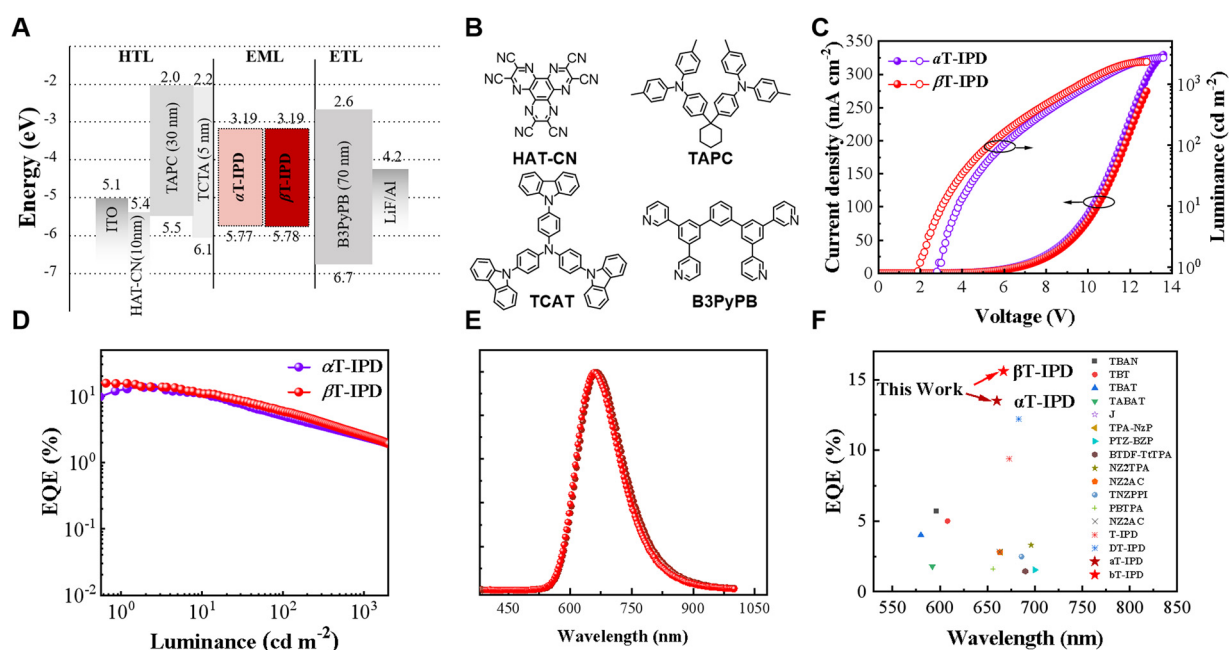
Fig. 4 (A) OLED structure, HOMO and LUMO energy diagram. (B) The material structure used in the functional layer, (C) current density ( J )–voltage ( V )–luminance ( L ) curves, (D) EQE– L curves, and (E) EL spectra of non-doped OLEDs based on \alpha T-IPD and \beta T-IPD. (F) Reported representative hot exciton DR-OLEDs.
