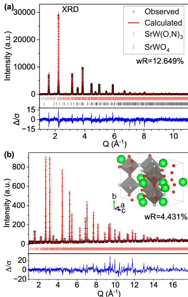
Fig. 4 Rietveld refinement of \text{SrW}(\text{O},\text{N})_3 (a) synchrotron XRD and (b) ND patterns using a 40-atom P1 structure suggested by our theory-based approaches (model S-III).
