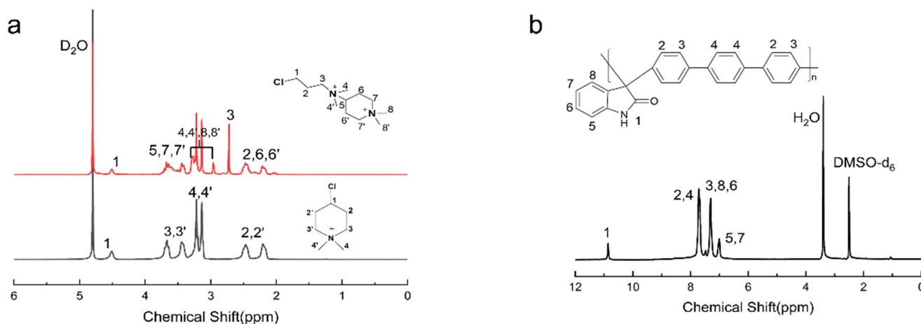
Fig. 1 1 H NMR spectra of (a) 4-ClPq and 3-N-4-CIPq; (b) poly(p-terphenyl isatin).
