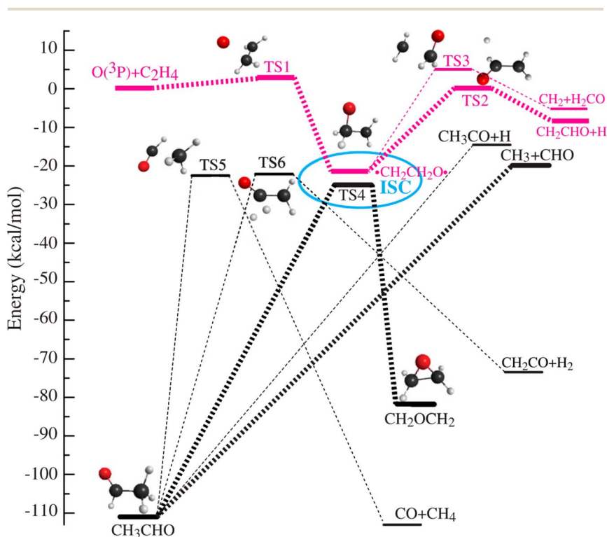
Fig. 4 Simplified schematic of triplet (red) and singlet (black) potentials of the O( 3 P) + C 2 H 4 reaction. The electrophilic oxygen atom attacks the C=C bond through a very low barrier of about 3 kcal mol -1 and forms an energetic triplet biradical, 'CH 2 CH 2 O'. The biradical region, enclosed by the ellipse, is where intersystem crossing (ISC) takes place with the greatest probability. ISC competes with fragmentation and rearrangement. The corresponding singlet biradical can isomerize to acetaldehyde (CH 3 CHO), which subsequently dissociates because of its high energy content. The triplet biradical can dissociate to H + CH 2 CHO or to CH 2 + H 2 CO. The singlet biradical can also isomerize to oxirane via oxygen migration and ring-closure. The oxirane will finally isomerize to CH 3 CHO and further dissociate from CH 3 CHO into various products, CH 3 + HCO, and H + CH 3 CO. Adapted from ref. 230.
