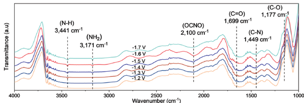
Fig. 15 Mechanistic investigations involving the formation of *ONCO using the Cu 1 –CeO 2 catalyst. Operando SR-FTIR spectroscopy measurements at different potentials during electroreduction of CO 2 and NO 3 - . Adapted from ref. 184.
