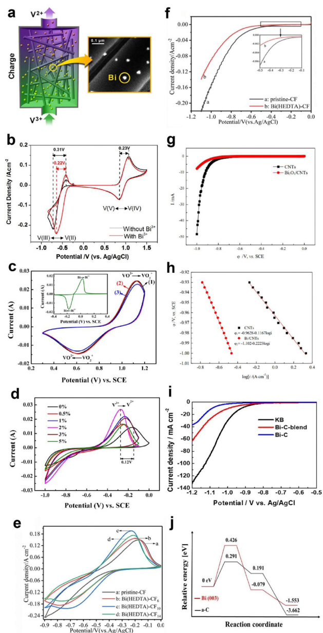
Fig. 6 (a) Depiction of Bi-loaded graphite felt utilization in VRFBs. (b) Cyclic voltammetry (CV) profiles on a glassy carbon electrode within 2 M VOSO 4 + 5 M HCl electrolytes, with and without 0.01 M BiCl 3 . Reproduced with permission from ref. 98. Copyright 2013 American Chemical Society. (c) CV curves: curves 1 and 2 corresponds to 0% and 2% Bi-loaded CF in 0.05 M VO 2+ + 0.05 M VO 2 + + 3 M H 2 SO 4 solution, respectively; and curve 3 corresponds to the 0% Bi-CF in the same solution. (d) CV curves of x-Bi-CF (x = 0%, 0.5%, 1%, 3%, 5%) in 0.05 M V 3+ + 0.05 M V 2+ + 3 M H 2 SO 4 solution are presented. Reproduced with permission from ref. 99. Copyright 2017 Elsevier. (e) CV profiles of pristine-CF and Bi(HEDTA)-CFs acquired in a 3 mol L -1 V 3+ + 3 mol L -1 H 2 SO 4 solution. (f) LSV curves of pristine and Bi(HEDTA)-CF 10 tested in a 1 mol L -1 H 2 SO 4 solution at a scan rate of 2 mV s -1 . Reproduced with permission from ref. 101. Copyright 2019 Springer. (g) and (h) LSV curves and Tafel plots for bare carbon nanotubes (CNTs) and Bi 2 O 3 /CNTs electrodes assessed in a 3 mol L -1 H 2 SO 4 solution with a scan rate of 1 mV s -1 . Reproduced with permission from ref. 102. Copyright 2020 ESG. (i) LSV curves of Ketjenblack (KB), Bi-C blend, and aC surfaces. (j) Density functional theory (DFT) generated free energy diagrams depicting associative HER pathways on Bi(003) and aC surfaces. Reproduced with permission from ref. 40. Copyright 2023 Elsevier.
