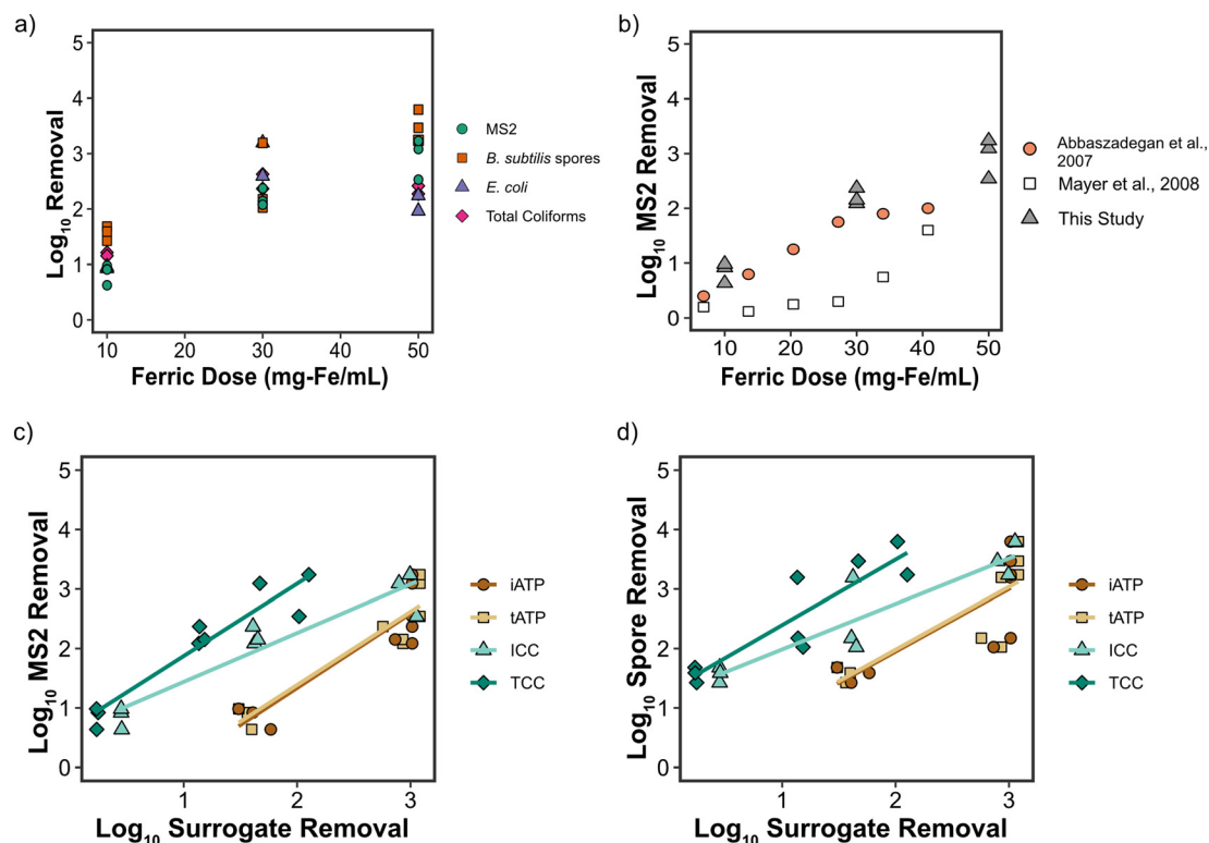
Fig. 4 \log_{10} removals of spiked microorganisms (a) MS2 bacteriophage, B. subtilis spores, E. coli , and total coliforms with increasing ferric chloride dose; (b) MS2 bacteriophages with increasing ferric chloride doses compared to other bench-scale spiking studies; and (c) MS2 bacteriophage and (d) B. subtilis spore removal with respect to removals of rapid microbial surrogate parameters.
