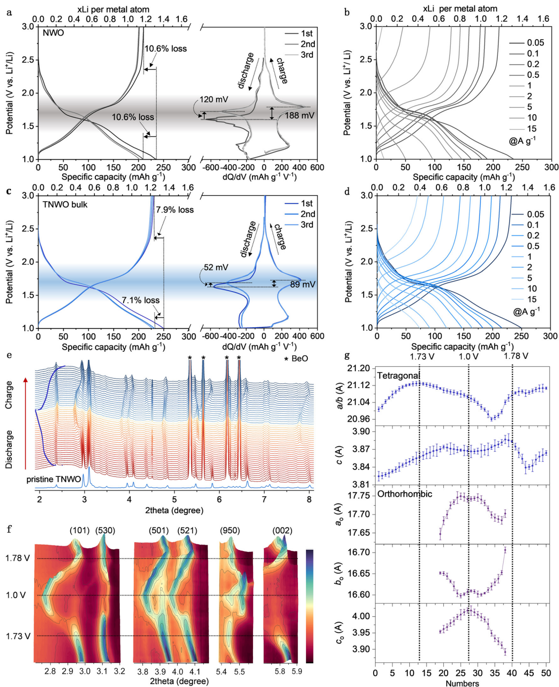
Fig. 3 Electrochemical Li + storage behaviors of NWO bulk and TNWO bulk anodes in coin-type half cells. (a) and (c) GCD curves at 0.05 A g -1 and corresponding dQ/dV plots ( Q : capacity; V : potential) for initial three cycles. (b) and (d) Initial GCD curves at current densities ranging from 0.05 A g -1 to 15 A g -1 . (e)–(g) Operando high-energy synchrotron XRD patterns and the corresponding GCD curve, contour plots and refined lattice parameter evolution during the initial (d)lithiation process of the TNWO bulk anode.
