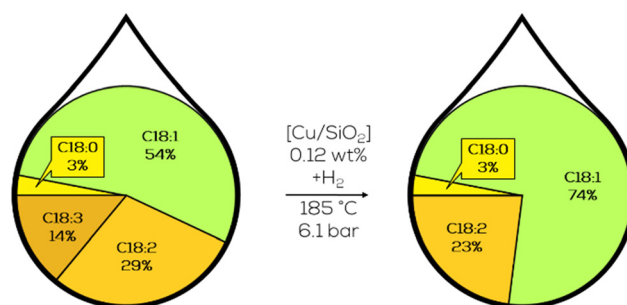
Fig. 13 C18 fatty acid composition in the hydrogenation of canola oil with heterogeneous copper catalysts immobilized on SiO 2 as performed by Johannson et al. 97
