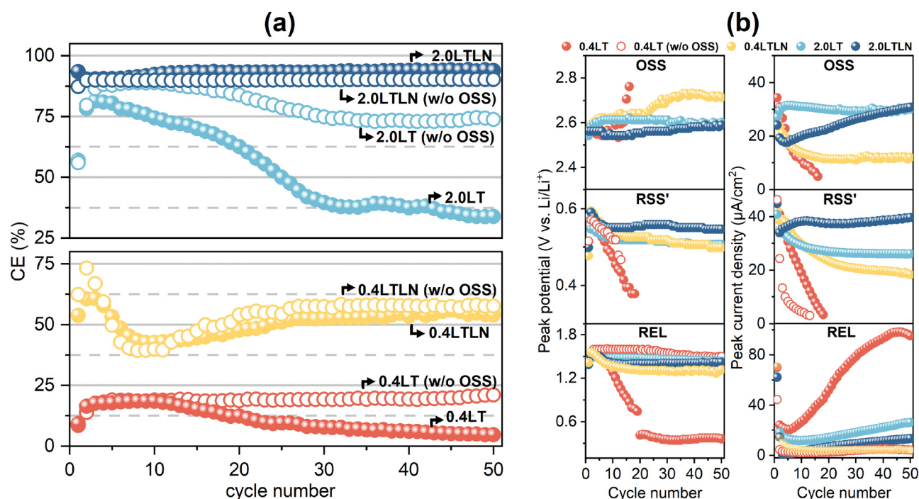
Fig. 2 (a) 50-Cycle CE performances in 0.4LT, 0.4LT/LN, 2.0LT and 2.0LT/LN (with and w/o the occurrence of OSS); (b) cycling dependence of the peak potential and peak current density of OSS, RSS' and REL obtained from CV measured in 0.4LT, 0.4LT w/o OSS, 0.4LT/LN, 2.0LT and 2.0LT/LN.
