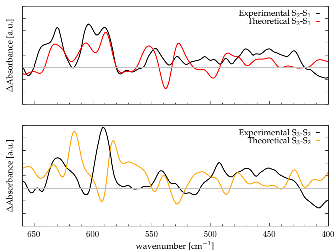
Fig. 3 Differential spectra obtained with theoretical IR intensities (red and orange lines) compared with the experimental data (black lines) from ref. 46 ; the grey line corresponds to the zero of the differential spectrum. Top panel: S_2 -minus- S_1 ; bottom panel: S_3 -minus- S_2 .
