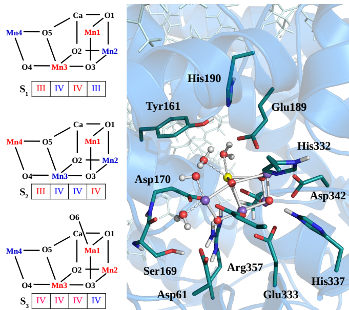
Fig. 1 Structural sketch of Mn 4 Ca cluster and the respective spin/redox for each studied state are shown in the left panel. In the right panels are shown the residues included in the QM region for all the QM/MM simulations.
