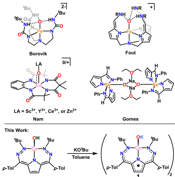
Scheme 1 Top: Examples of previously reported metal oxidos stabilized by hydrogen bonding or Lewis acid interactions. Bottom: Synthesis of 1 from [\text{tBu,TolDHP}]\text{CoOH} .
