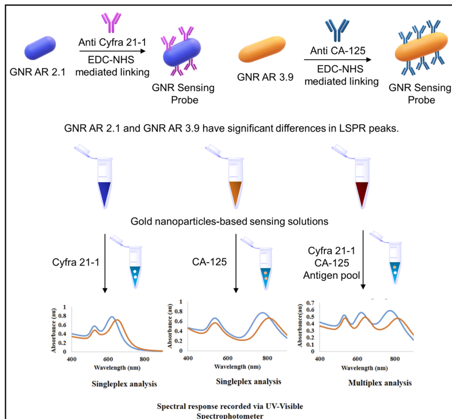
Fig. 13 The schematic depicting GNR probe development and the UV-visible spectroscopy-based spectral analysis of Cyfra 21-1 and CA-125 antigens. Reproduced/re-drawn with permission from ref. 153. Copyright 2022 The Royal Society of Chemistry.
