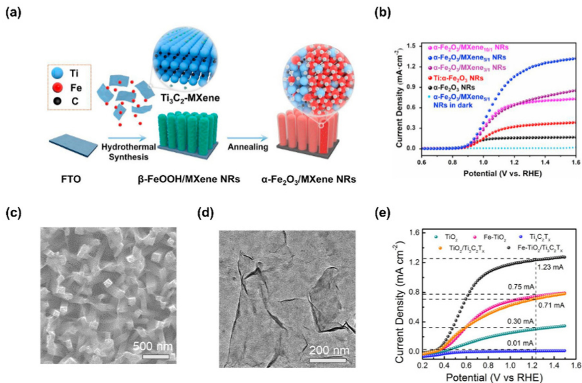
Fig. 11 (a) Schematic of fabrication process for \alpha\text{-Fe}_2\text{O}_3/\text{MXene} , NRs. (b) LSV curves \alpha\text{-Fe}_2\text{O}_3 , NRs, \text{Ti}_3\text{-Fe}_2\text{O}_3 , \alpha\text{-Fe}_2\text{O}_3/\text{MXene}_{5/1} NRs, \alpha\text{-Fe}_2\text{O}_3/\text{MXene}_{10/1} NRs, and \alpha\text{-Fe}_2\text{O}_3/\text{MXene}_{10/1} NRs. Copyright 2021, Elsevier. (c) SEM image of the Fe- \text{TiO}_2/\text{Ti}_3\text{C}_2\text{T}_x . (d) TEM image of the exfoliated \text{Ti}_3\text{C}_2\text{T}_x nanosheets. (e) LSV curves of \text{TiO}_2 , \text{Ti}_3\text{C}_2\text{T}_x , \text{TiO}_2/\text{Ti}_3\text{C}_2\text{T}_x , Fe- \text{TiO}_2 (Fe: 5 mol%) and Fe- \text{TiO}_2/\text{Ti}_3\text{C}_2\text{T}_x . Copyright 2022, Elsevier.
