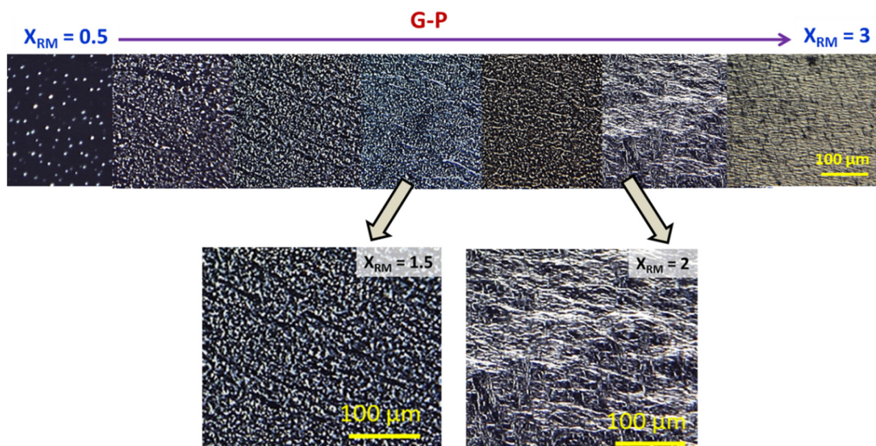
Fig. 1 POM images taken in the isotropic for samples polymerised in gel phase (G-P) with varied concentrations of photopolymer ( X_{RM} ). Droplet morphology was seen for lower X_{RM} , and improved the connectivity of the polymer strands was observed with the increase in the monomer concentration. Although enlarged images (below) display well-connected polymer networks at higher X_{RM} , the networks are more distorted; a consequence of the surrounding nematic-gel environment.
