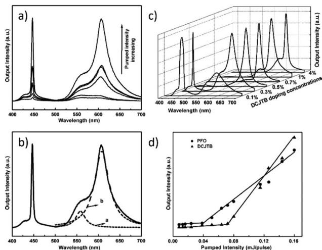
Fig. 23 (a) Normalized emission spectra of the DCJTBT:PFO thin film (DCJTBT doped concentration is 0.3%) at different pumped intensities. (b) The broadband emission from 530 to 680 nm consists of two peaks. (c) ASE spectra of DCJTBT:PFO thin film with different doping concentrations of DCJTBT at the pumped intensity of 0.12 \text{ mJ pulse}^{-1} . (d) Output emission intensity of the DCJTBT:PFO film at the peak wavelength of 446 and 605 nm as a function of the pumped intensity. Reproduced (or Adapted) with permission, 161 2008, American Institute of Physics.
