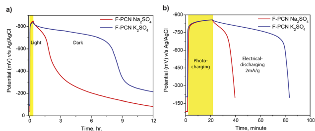
Fig. 4 (a) OCP measurement on F-PCN in the presence of different electrolytes ( M_2SO_4 and 4-MBA) (b) Photo charging of F-PCN in the presence of different electrolytes for 20 minute (OCP) and subsequently electrical discharging with 2 \text{ mA g}^{-1} . All the measurements are done in an inert condition.
