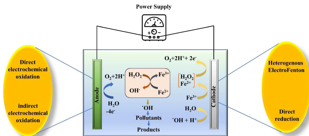
Fig. 2 Schematic illustration of the electro-Fenton process.
