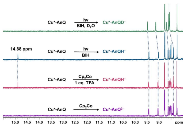
Fig. 7 Comparison of the ^1\text{H} NMR spectra of \text{Cu}^+\text{-AnQ}^{\bullet-} (purple line), \text{Cu}^+\text{-AnQH}^{\bullet-} generated by \text{Cp}_2\text{Co} and 1 eq. trifluoroacetic acid (red line), \text{Cu}^+\text{-AnQH}^{\bullet-} generated by 30 minutes illumination with BIH (teal line), \text{Cu}^+\text{-AnQ}^{\bullet-} generated by BIH with 30 min illumination and then added with one drop of \text{D}_2\text{O} (green line). Illumination with 455 nm light; concentrations of the complex and BIH were kept at 0.2 mM and 0.1 M, respectively, in \text{CD}_3\text{CN} .
