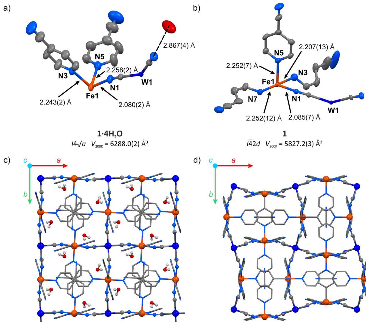
Fig. 2 Structural transformation accompanying the transition from 1 ·4H 2 O to 1 : asymmetric unit of 1 ·4H 2 O (a) and 1 (b) with selected bond distances (hydrogen atoms were omitted for clarity), as well as coordination frameworks of 1 ·4H 2 O (c) and 1 (d) as seen along the crystallographic c -axis (hydrogen atoms of 4-cyanopyridine molecules were omitted for clarity). W – dark blue, Fe – orange, O – red, N – blue, C – grey.
