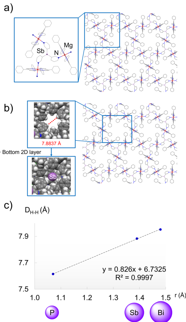
Fig. 7 (a) X-ray structure showing the 2D polymeric arrangement of 1 \cdot Mg . Pyridyl coordination at both axial positions of MgTPP results in an extended structure. The inset shows the capsule that results from the coordination of 1 to three MgTPP units. H atoms and CHCl_3 solvent molecules are omitted for clarity. Selected bond lengths (Å) and angles (°): 1 \cdot Mg , Sb-C_{py} 2.155(4); N_{py}-Zn 2.330(2); C_{py}-Sb-C_{py} 94.6(2). Colour key: C (grey), N (blue), Sb (light purple), Mg (red). (b) X-ray structure of the 2D polymeric structure of 1 \cdot Mg showing the 2-D network structure consisting of Sb_6Mg_6 ring units, which leads to the formation of hexagonal voids in the structure (inset). (c) Linear correlation between the covalent radii of the bridgehead atom and the effective size of the hexagonal voids ( D_{H-H} ) in the X-ray structures of P \cdot Mg , 1 \cdot Mg and 2 \cdot Mg . Colour key: C (grey), N (blue), Sb (light purple), Mg (red).
