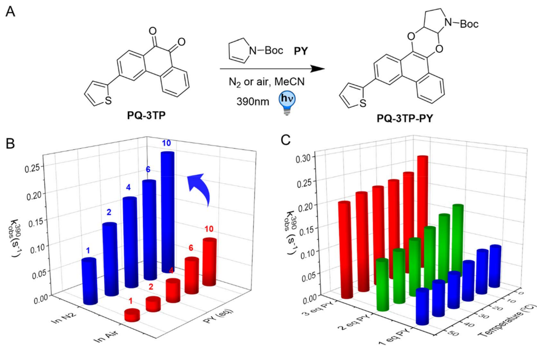
Fig. 3 Kinetic analysis of PQ-3TP 2 PY photoclick reaction. (A) Reaction scheme (one of the possible isomers formed is shown as an example), (B) kinetic analysis of photocycloaddition between PQ-3TP (50 \mu M) with varying amounts of PY (1, 2, 4, 6, and 10 eq.) addition under both N 2 (blue cylinders) and air (red cylinders) atmosphere at 20 ^{\circ} C. (C) Temperature dependence kinetic analysis of PQ-3TP 2 PY photoclick reaction in MeCN under different temperature 0 ^{\circ} C, 10 ^{\circ} C, 20 ^{\circ} C, 30 ^{\circ} C, 40 ^{\circ} C, and 50 ^{\circ} C respectively. For all of the measurements, the sample was irradiated with a 390 nm LED and followed over time by UV-Vis absorption spectroscopy (1 cm cuvette, 2.5 mL MeCN sample volume, sample interval 1 s).
