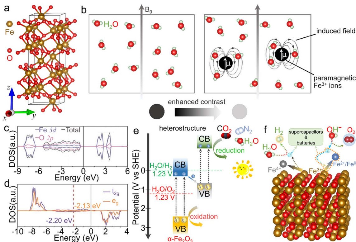
Fig. 2 Crystal structure and basic physicochemical characteristics of the \alpha\text{-Fe}_2\text{O}_3 phase. (a) Crystal structure of the rhombohedral \alpha\text{-Fe}_2\text{O}_3 phase, in which brown and red balls represent iron and oxygen atoms, respectively. (b) Scheme for the enhanced T_1 -weighted magnetic resonance contrast induced by paramagnetic ions, wherein B_0 represents an external field. (c) Density of states (DOS) and (d) projected DOS on the spin orbitals of t_{2g} and e_g of Fe atoms. (c and d) Adapted with permission from ref. 54. Copyright 2019, John Wiley & Sons, Inc. (e) Scheme of an \alpha\text{-Fe}_2\text{O}_3 -based heterostructure for photocatalysis. (f) Scheme for the redox properties of \alpha\text{-Fe}_2\text{O}_3 for energy-related applications.
