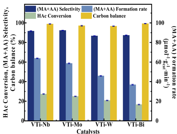
Fig. 8 Catalyst performance of metal cation-doped VPO catalysts. The reaction temperature and carrier flow rate was 360^\circ\text{C} and 50 \text{ mL min}^{-1} (3.0 vol% O 2 in N 2 ), respectively. The liquid feed was a HAc-FA mixture (2.5/1, n/n ), with a LHSV of 1.33 \text{ mL h}^{-1} \text{ g}_{\text{cat}}^{-1} .
