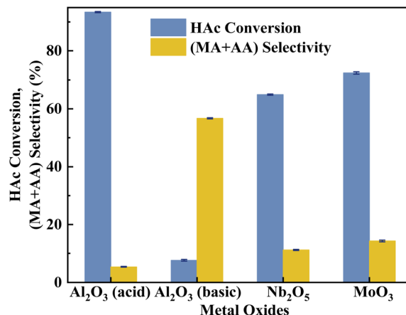
Fig. 9 Catalyst performance of metal oxides. The reaction temperature and carrier flow rate was 360^\circ\text{C} and 50 \text{ mL min}^{-1} (3.0 vol% O 2 in N 2 ), respectively. The liquid feed was a HAc-FA mixture (2.5/1, n/n ), with a LHSV of 1.33 \text{ mL h}^{-1} \text{ g}_{\text{cat}}^{-1} .
