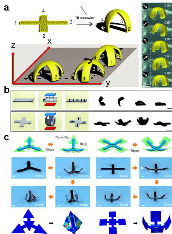
Fig. 15 The magnetic-responsive shape morphing behavior of composite hydrogels. (a) Schematic representation of the hydrogel robotics rotating its body 90° counter-clockwise when the rotation direction of the magnetic field changes due to the addition of Ni nanowire from the y - z plane to the x - z plane. Reproduced with permission. 356 Copyrights 2020, American Association for the Advancement of Science. (b) PNaAMPS/NdFeB composite hydrogel is programmed with a NdFeB magnet and actuated using a static magnetic field in the form of a permanent magnet inducing a shape change. Scale bars are 10 mm. 354 Reproduced with permission. Copyrights 2021, Royal Society of Chemistry. (c) Fe 3 O 4 /PNIPAM is actuated with an alternating magnetic field causing a shape change. Scale bars are 5 mm. Reproduced with permission. 189 Copyrights 2019, American Chemical Society.
