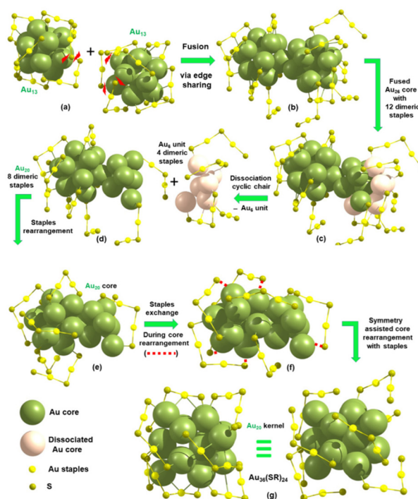
Scheme 4 The proposed mechanism for cluster transformation. (a and b) Scissoring dimeric staples in \text{Au}_{25}(\text{SR})_{18} clusters during fusion. (c, d and e) Dissociation of the cyclic chair conformation of the \text{Au}_6 unit from the fused \text{Au}_{26} core and staples rearrangement. (f and g) Isomeric core transition via the complex core rearrangement process towards the more symmetric \text{Au}_{20} kernel structure forming \text{Au}_{36}(\text{SR})_{24} . The ligands are omitted for visual convenience.
