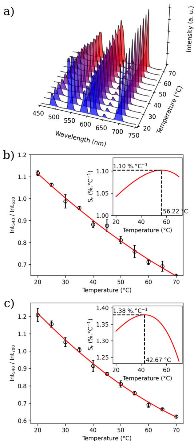
Fig. 5 (a) Emission spectra ( \lambda_{\text{exc}} = 312 \text{ nm} ) of MSN-1 recorded at different temperatures ranging from 20 to 70 °C in water; (b) the corresponding LIR between the ^5\text{D}_4 \rightarrow ^7\text{F}_5 ( \text{Tb}^{3+} ) and ^5\text{D}_0 \rightarrow ^7\text{F}_2 ( \text{Eu}^{3+} ) transitions. The solid line represents a second-degree polynomial fitting. Integrated areas: 530–560 nm ( \text{Tb}^{3+} : ^5\text{D}_4 \rightarrow ^7\text{F}_5 ) and 604–642 nm ( \text{Eu}^{3+} : ^5\text{D}_0 \rightarrow ^7\text{F}_2 ). Insert: temperature dependence of S_r . Inset: temperature dependence of S_r . The error bars correspond to the standard error of the mean determined from three consecutive temperature cycles.
