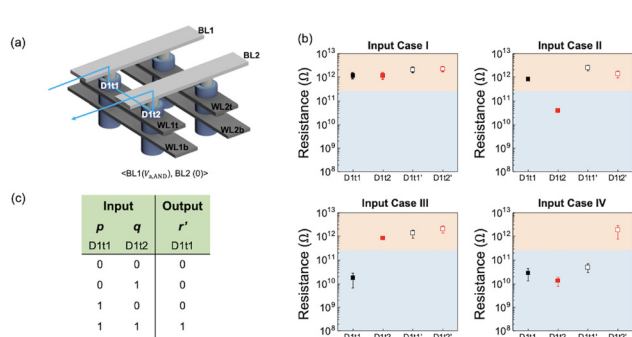
Fig. 5 Experimental demonstration of the AND logic gate between D_{11t} and D_{112} memristors in the BLC. (a) The bias configuration in the schematic diagram of the vertical CBA, where V_{a,\text{AND}} = +9 V. (b) The results of the AND logic operation in D_{11t} for each input case. A resistance lower than 250 G \Omega is encoded to the “1” state and (c) its truth table of the logic gate.
