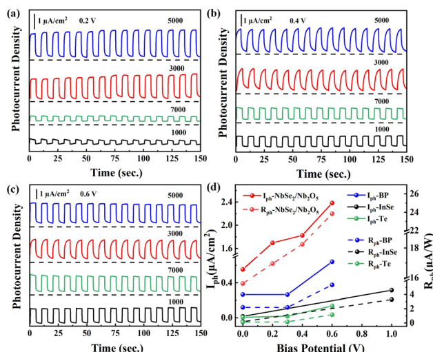
Fig. 5 Time-dependent photocurrent density of \text{NbSe}_2/\text{Nb}_2\text{O}_5 under the different centrifugal speed (1000, 3000, 5000, and 7000 rpm)-based PEC photodetectors was measured at (a) 0.2 V, (b) 0.4 V, and (c) 0.6 V; (d) I_{\text{ph}} and R_{\text{ph}} values of the 2D material-based PEC-type photodetector, including \text{NbSe}_2/\text{Nb}_2\text{O}_5 (this work), BP, 41 InSe, 43 and Te. 42
