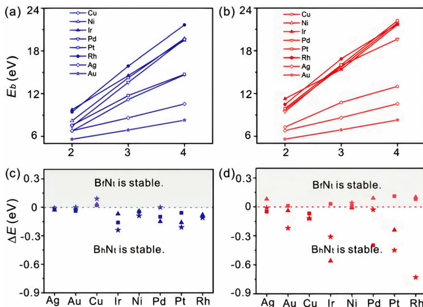
Fig. 3 Binding energies as a function of BN clusters terminated with (a) N and (b) B atoms. The difference in formation energy between B_hN_t and B_rN_t of (c) N and (d) B terminated BN clusters. Squares, stars, and triangles represent the cluster size of 2, 3, and 4, respectively. 180
