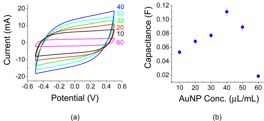
Fig. 4 (a) Successive C - V plots for various concentrations (in units of \mu\text{L} of Au per mL of solvent appearing on the side) depicted on the right. (b) Capacitance as a function of AuNP concentration exhibits a peak at 40 \mu\text{L mL}^{-1} . The electrolyte was 1 M of \text{Na}_2\text{SO}_4 .
