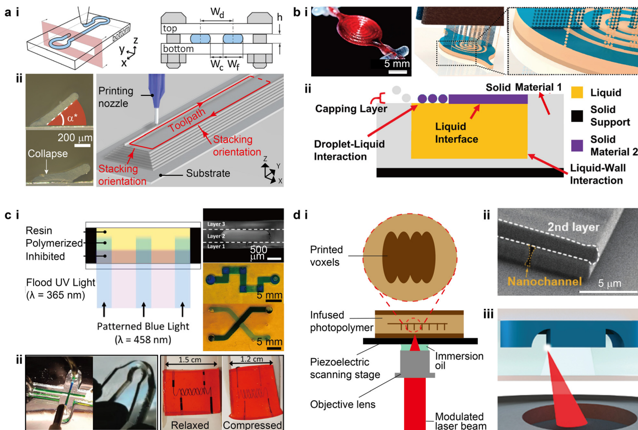
Fig. 2 Advances in the strategies for 3D printing microfluidic devices. (a) Extrusion-based 3D printing. (i) Schematic of extruding room temperature-curable silicone inks on flat substrates that are subsequently enclosed by a top cover. W_d , W_c , W_f , and h denote the design width, channel width, filament width, and channel height, respectively. (ii) Images of printing silicone thin walls and a schematic of printing microfluidic channels. \alpha^* denotes the critical angle above which the printed walls could maintain their equilibrium states. (b) PolyJet printing. (i) Conceptual schematic illustrating the PolyJet printing of a fluidic capacitor consisting of building material (blue) and temporary supporting material (beige). The image shows a completed capacitor. (ii) Schematic of the solid-liquid co-printing process where liquid-wall and droplet-liquid interactions were involved. The printing heads and UV light source are not shown. (c) Stereolithography. (i) Left: Schematic of a variation of dual wavelength SL. Right: Optical images of SL printed multi-layer microstructures, serpentine channels, and crossing channels. (ii) Left: SL printed PDMS-based microfluidic channels with a width of 500 \mu\text{m} and a bent dog-bone specimen. Right: SL printed 2-phenoxyethyl acrylate-based soft microfluidic device containing helical channels with a width of 200 \mu\text{m} . (d) Direct laser writing. (i) Typical configuration of a DLW printing stage. The magnified view illustrates a sequence of cured voxels. (ii) SEM micrograph of a nanoscale channel printed by DLW. (iii) Schematic of in situ direct laser writing, where the focused laser prints encased structures within a microfluidic channel. (a-i) Was adapted with permission from ref. 8. (a-ii) Was adapted with permission from ref. 13. (b-i) Was adapted with permission from ref. 29. (b-ii) Was adapted with permission from ref. 30. (c-i) Was adapted with permission from ref. 44. (c-ii) Was adapted with permission from ref. 53 (left) and ref. 54 (right). (d-ii) Was adapted with permission from ref. 60. (d-iii) Was adapted with permission from ref. 16.
