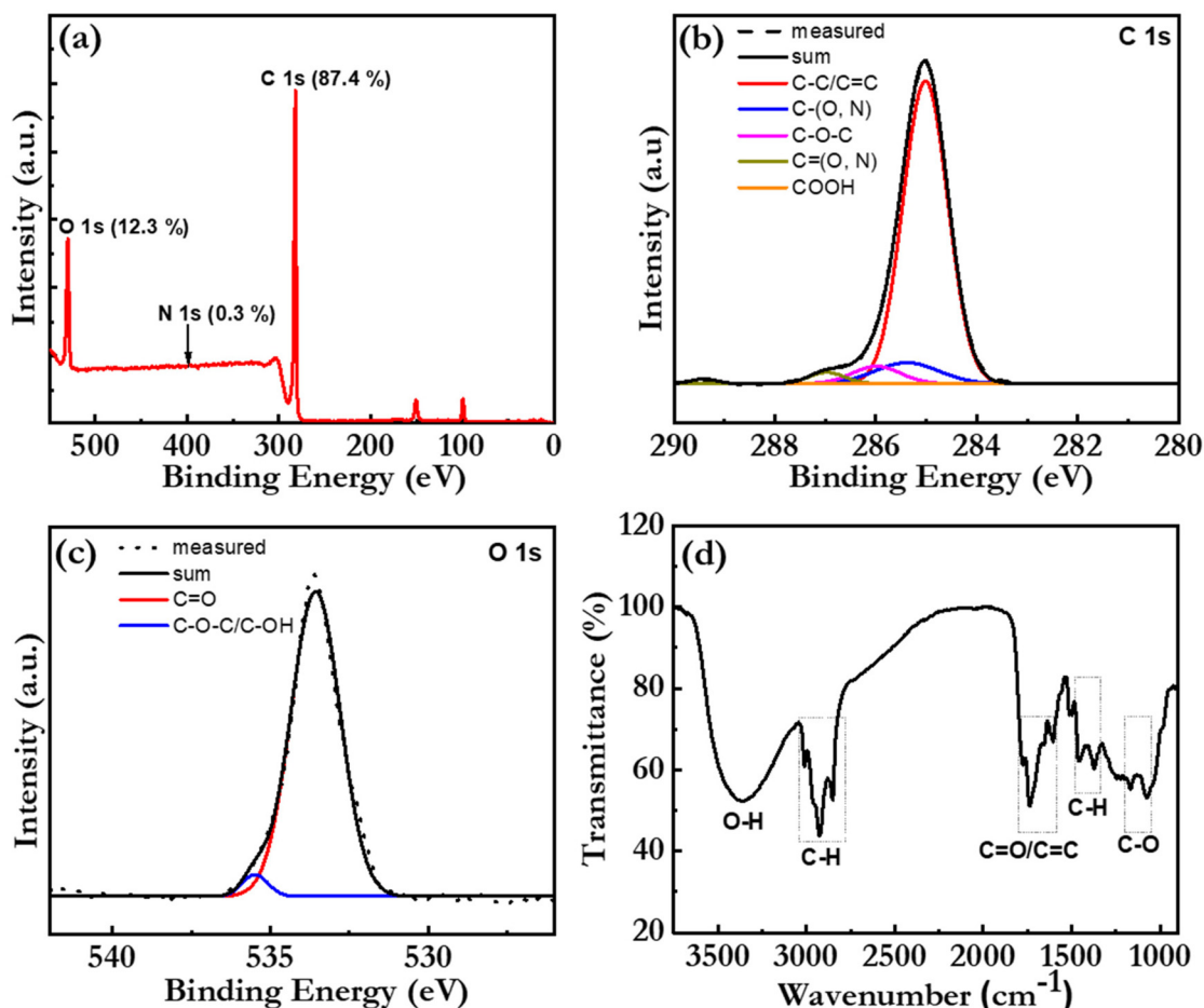
Fig. 3 (a) The XPS survey spectrum of a 200 \mu\text{m} thick bio-CD film on a Si substrate. (b and c) The measured high-resolution XPS spectrum (dotted grey line) and the fitted XPS spectra in (b) the C 1s region and (c) the O 1s region. The chemical assignments and the sum of the fit spectra are identified in the insets. (d) The FTIR spectrum of a dry bio-CD powder, with the key vibrational peaks identified by the dashed black rectangles.
