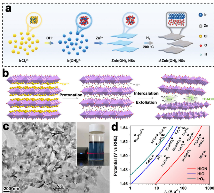
Fig. 5 (a) Schematic illustration of the synthesis of \text{ZnIr(OH)}_6 NSs and \text{ZnIr(OH)}_6 NSs (reproduced from ref. 92 with permission from the Royal Society of Chemistry, copyright 2022). 92 (b) Liquid-phase exfoliation of \text{Sr}_2\text{IrO}_4 . (c) TEM image of HION and the inset showing the photograph of HION colloidal suspension with typical Tyndall light scattering under laser irradiation. (d) Comparison of Ir mass activity of HION with previously reported OER catalysts in acid media (reproduced from ref. 93 with permission from the American Chemical Society, copyright 2022). 93
