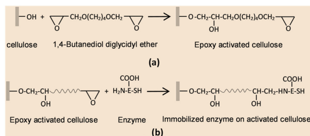
Fig. 10 Plausible reaction mechanism of enzyme immobilization through the epoxy method. (a) Surface reaction of a cellulose matrix with 1,4-butanediol diglycidyl ether (BTDE). (b) Covalent coupling of enzyme onto the surface of activated cellulose. Reproduced from ref. 54 with permission from Elsevier, copyright 2018.
