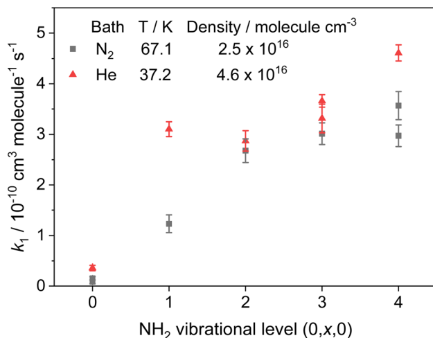
Fig. 4 Rate coefficients for the removal of NH 2 ( \nu = 0-4 ) with CH 3 CHO. Grey squares; T = 67.1 K, [\text{N}_2] = 2.5 \times 10^{16} molecules per cm 3 . Red triangles; T = 37.2 K, [\text{He}] = 4.6 \times 10^{16} molecules per cm 3 .
