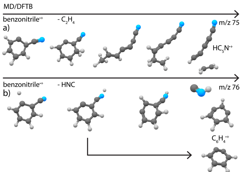
Fig. 8 Exemplary pathways for loss of (a) \text{C}_2\text{H}_4 and (b) \text{HNC} from canonical benzonitrile ^{+} as observed in the MD/DFTB simulations at 8.8 eV internal energy of the respective cation using Set1 parameters. The arrows indicate time.
